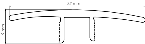
402 - Cover Trims for equal levels
